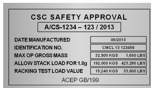
Figure 8.2 CSC safety approval plate with ACEP mark
